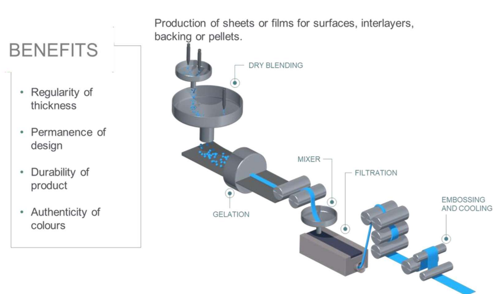
Figure 9: Calendering process
