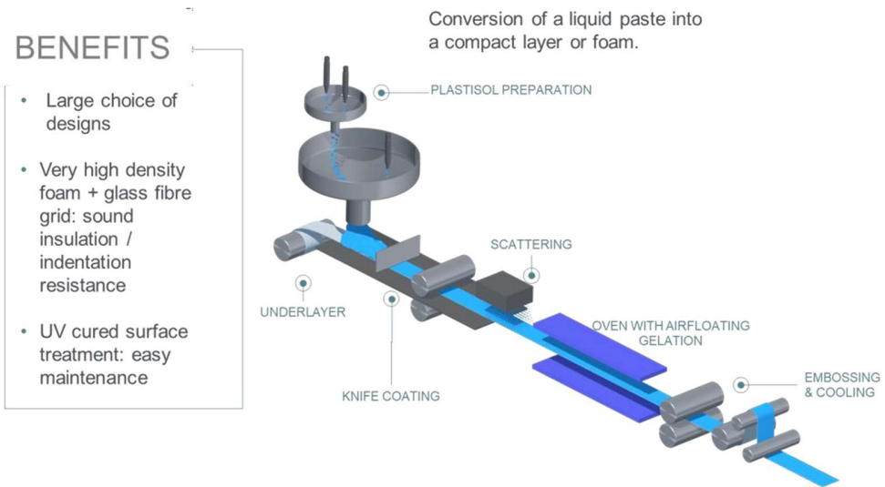
Figure 8: Coating process
